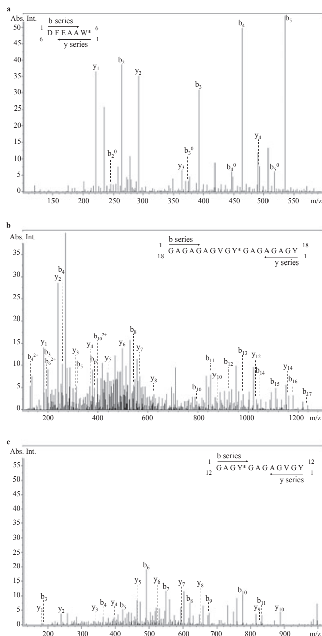
Figure 1. MS/MS spectra of: (a) monocharged peptide DFEAAW, m/z 754.304 with single oxidation from SA, (b) doubly charged peptide GAGAGAGVGYGAGAGY, m/z 708.336 with double oxidation from SA and (c) monocharged peptide GAGYAGAGVGY, m/z 1013.428 with quinone oxidation from PA.
