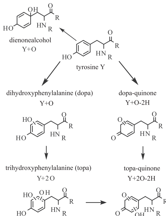
Figure 2. Tyrosine photo-oxidative pathway (44).
