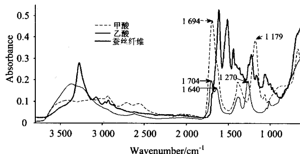
Fig. 1 FTIR spectra of pollutants and silk fabric
