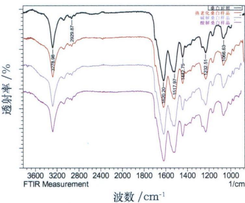
图 2 老化后白色桑蚕丝红外光谱图 Fig.2 FTIR spectra of aged white silkworm
