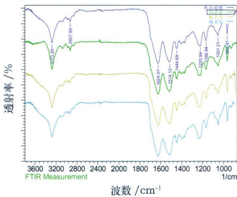
图 3 老化后柞蚕丝的红外光谱图 Fig.3 FTIR spectra of aged white tussah
