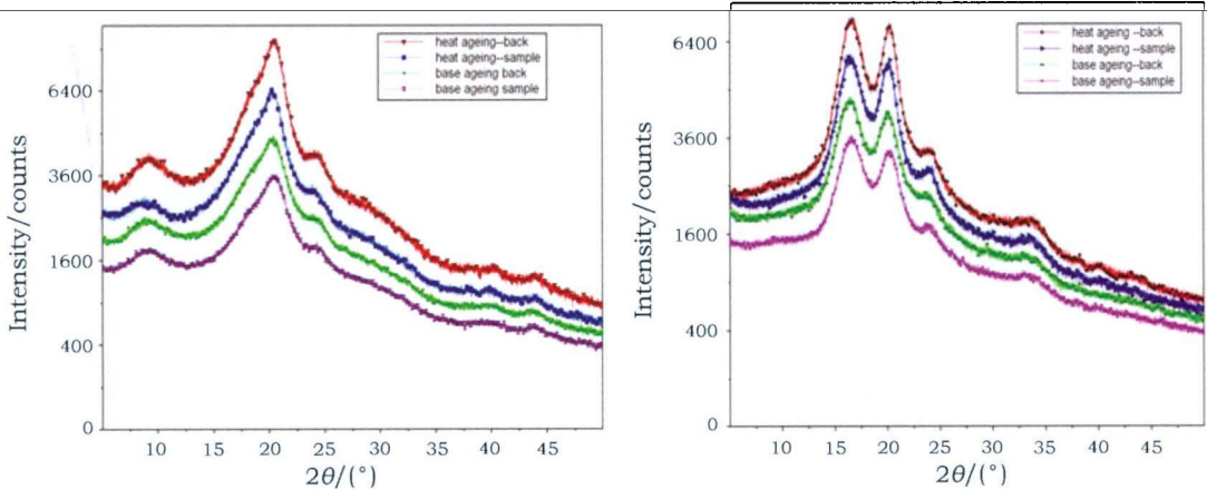
图 4 老化丝纤维 XRD(a 白色桑蚕丝,b 白色柞蚕丝) Fig.4 XRD results of aged sample(a is white silkworm,b is white tussah)
